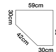
Corner Display Unit 3829/6829 H:188cm (74") Mirrors as standard
